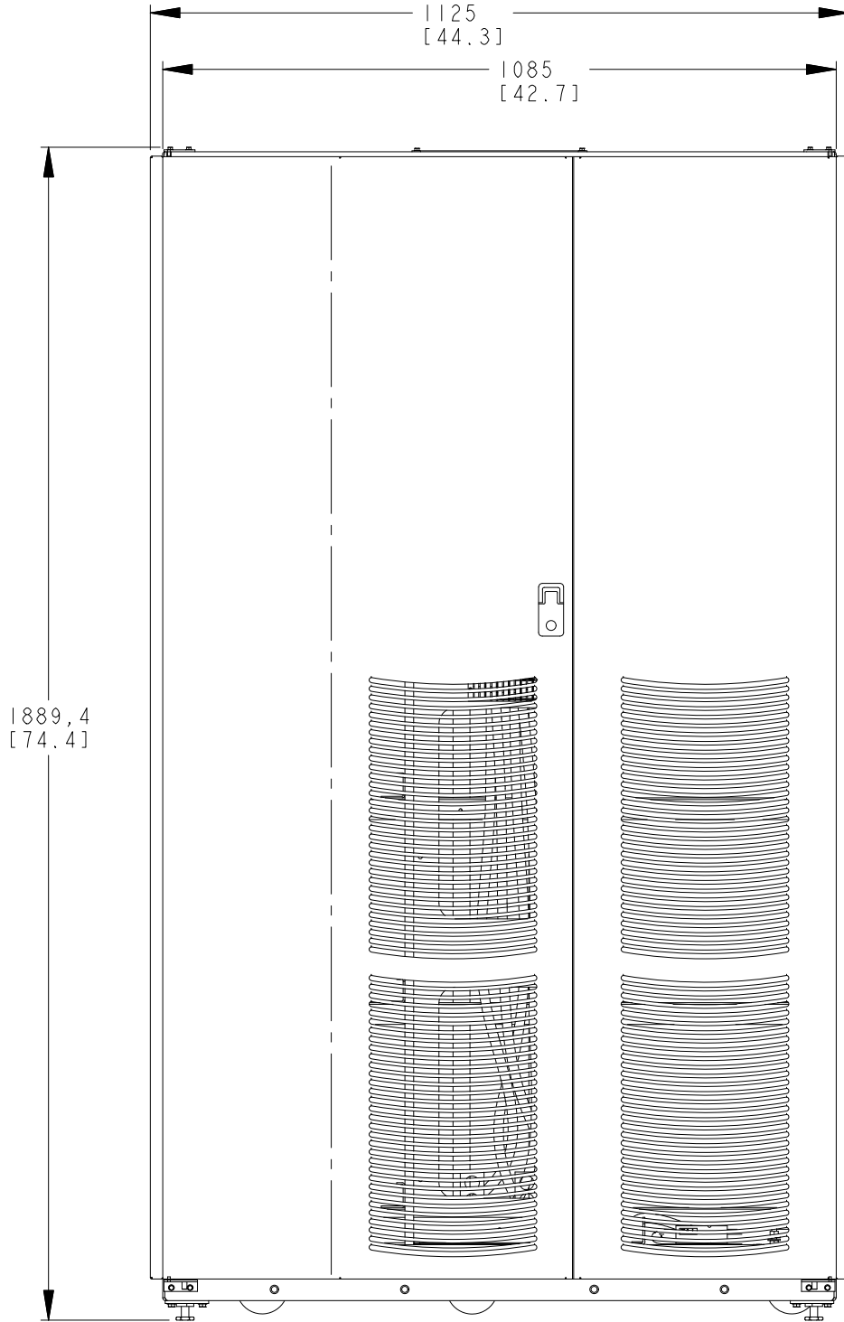
FRONT VIEW
