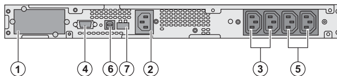
Evolution 1550 Rack
